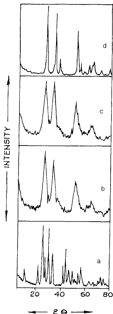
Fig. 1. XRD patterns of a) \text{La}_2\text{O}_3 , b) STL, c) \text{SO}_4^{2-}/\text{SnO}_2 , and d) \text{SnO}_2 calcined at 823 K.
